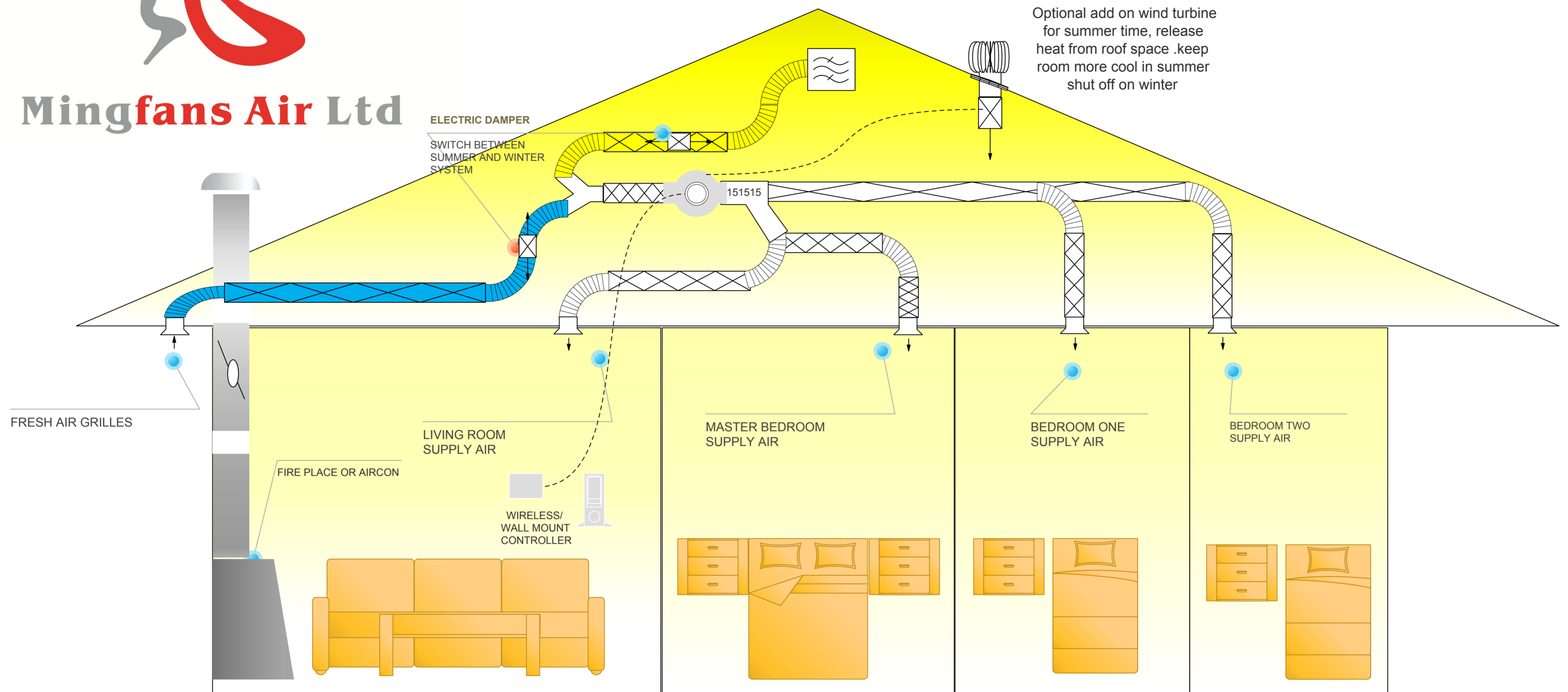
Optional add on wind turbine for summer time release heat from roof space .keep room more cool in summer shut off on winter
