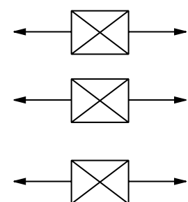
ELECTRIC DAMPER ROOF SPACE ELECTRIC DAMPER HEAT TRANSFER ELECTRIC DAMPER LIVING ROOM OPEN WHEN SUMMER KITS ON CLOSE WHEN HEAT TRANSFER ON
