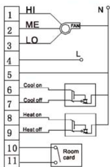
Heat /cool, 4 pipes, 3-wire valve control, fan coil unit system
